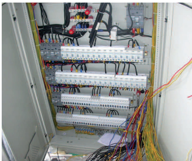
control board with MCB, MCCB and twin RCBO
